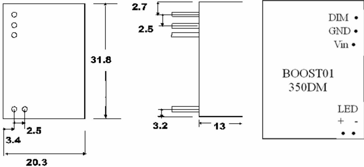
BOOST01-350DM (BOTTOM VIEW)
